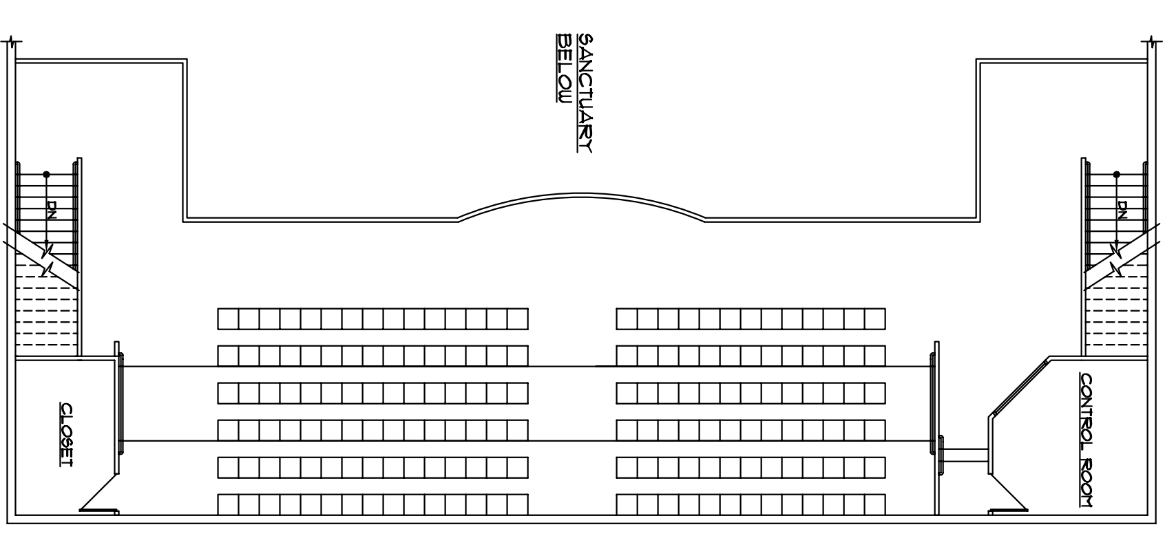
MEZZANINE PLAN 2,685 SF.
