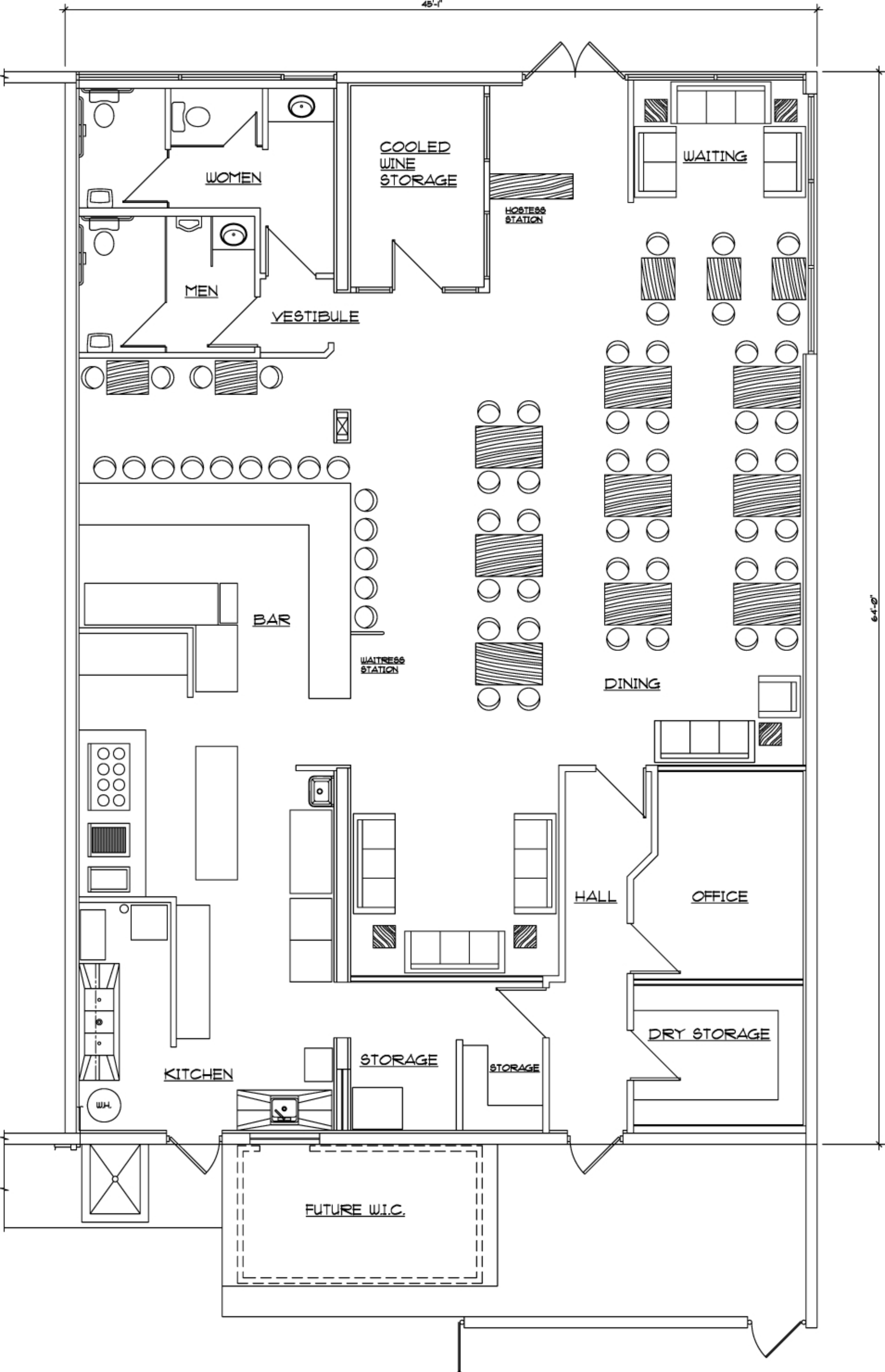
FLOOR PLAN 2,876 SF.
